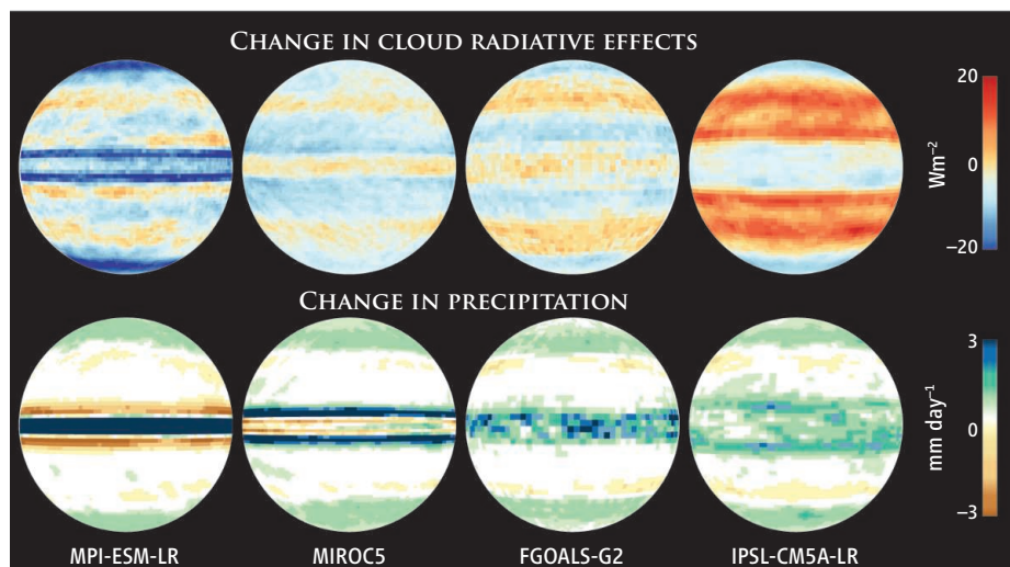
Wide variation. The response patterns of clouds and precipitation to warming vary dramatically depending on the climate model, even in the simplest model configuration. Shown are changes in the radiative effects of clouds and in precipitation accompanying a uniform warming (4°C) predicted by four models from Phase 5 of the Coupled Model Intercomparison Project (CMIP5) for a water planet with prescribed surface temperatures.
